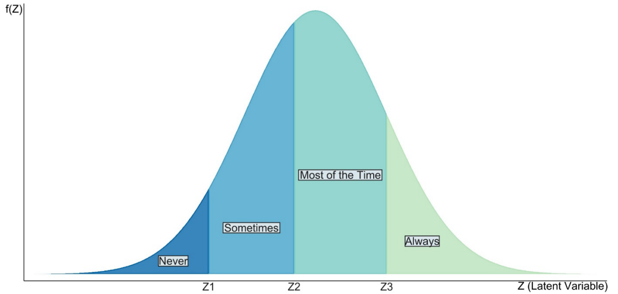
Figure 4: Z-scoring of categorical variables
