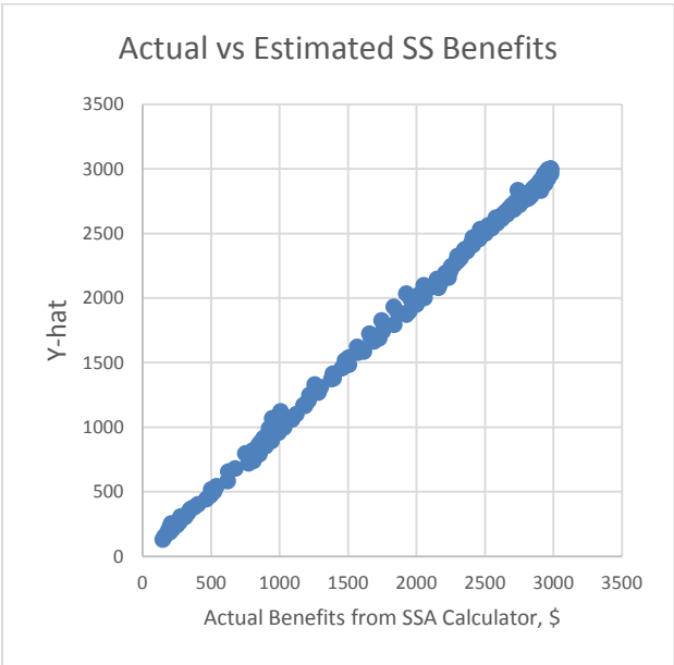
Figure A2. In-sample SS Benefits Model Performance
