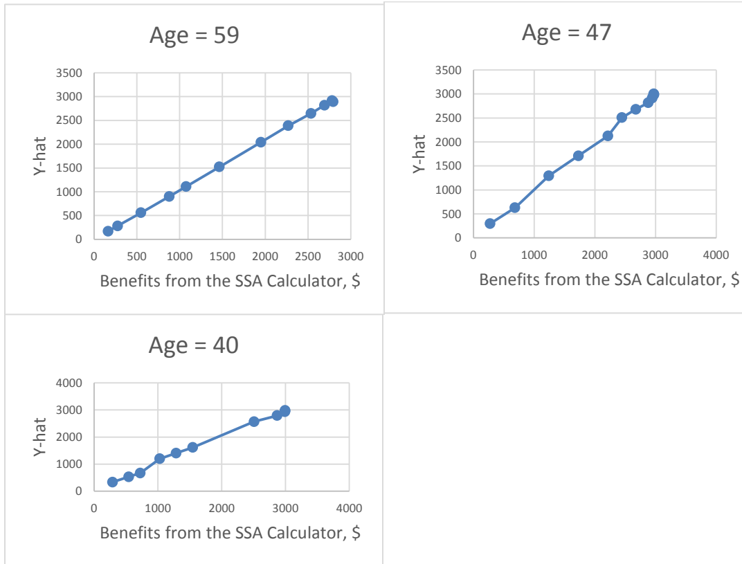
Figure 3A. Out-of-sample Model Performance for Three Ages
