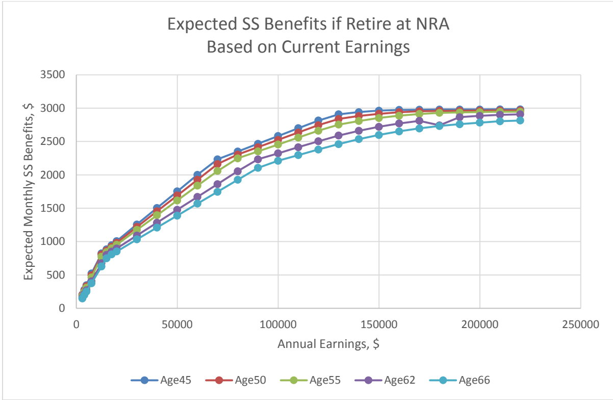
Figure A1. SSA Calculator Estimates of the SS Benefits at NRA
